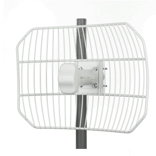
11"x14", 16dBi Antenna
